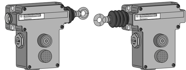
Fig. 1 Installation
